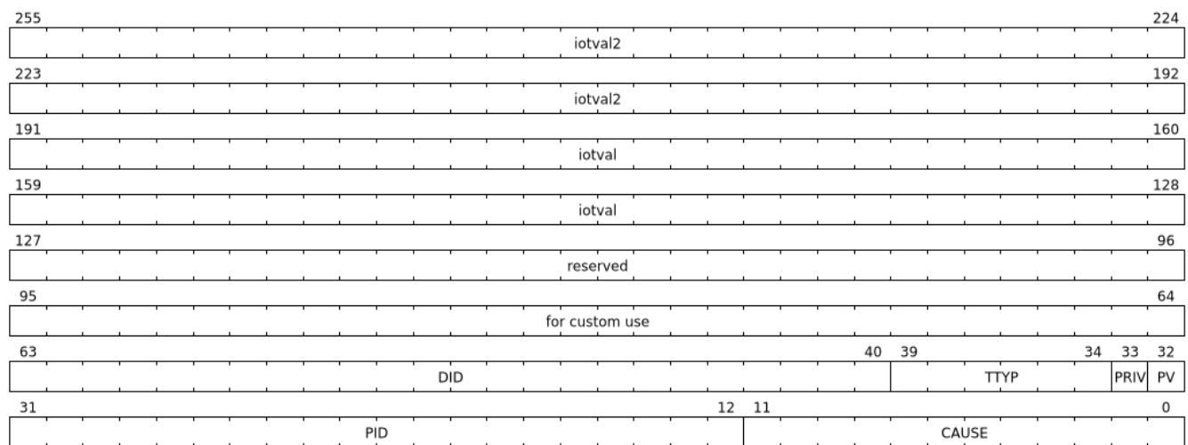
Figure 32. Fault-queue record
