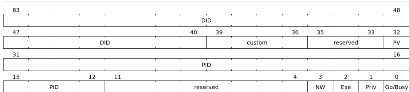
Figure 57. Translation-request control register fields
