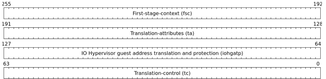
Figure 13. Base-format device-context
