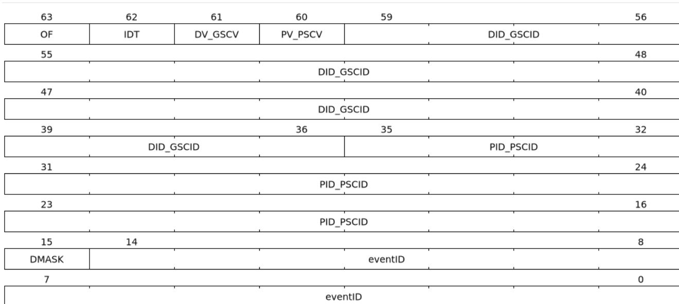
Figure 55. Performance-monitoring event selector register fields
