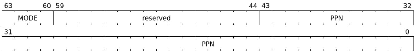
Figure 27. Process First-Stage context
