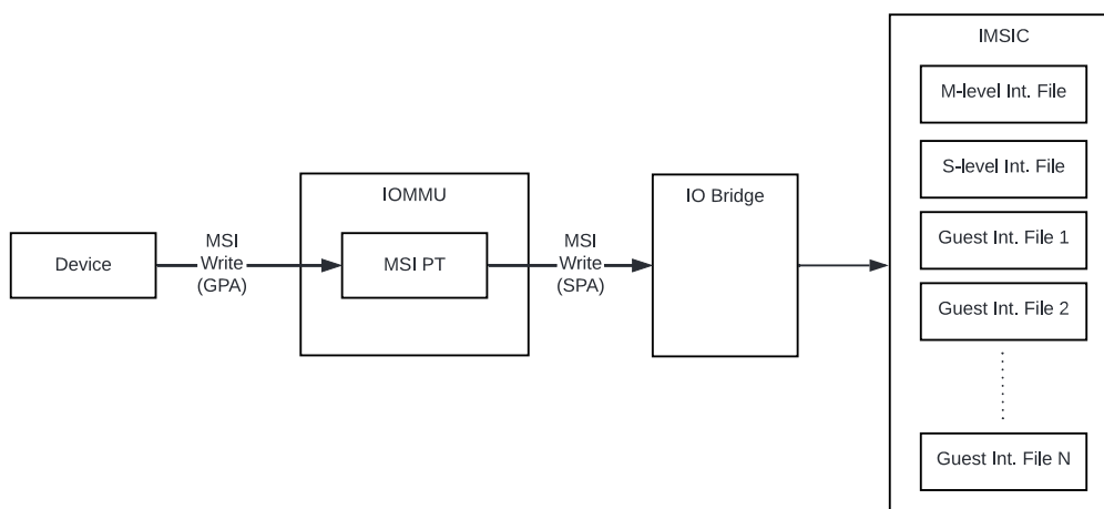
Figure 3. MSI address translation to direct guest programmed MSI to IMSIC guest interrupt files
