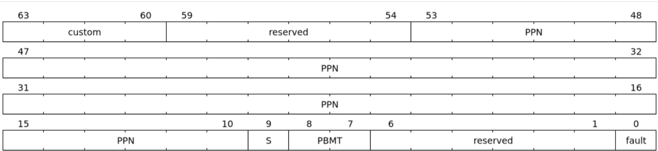
Figure 58. Translation-response register fields
