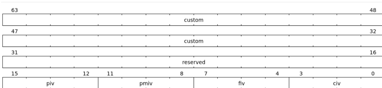
Figure 60. Interrupt-cause-to-vector register fields
